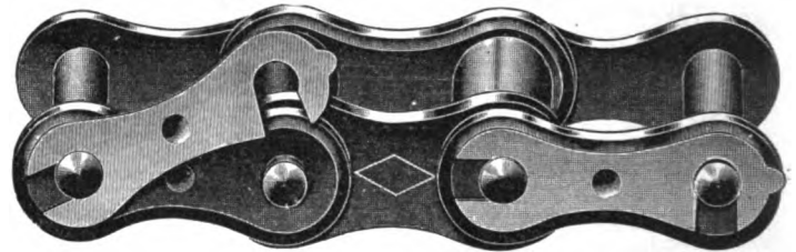
Diamond Detachable Chain Showing Locking Mechanism.
